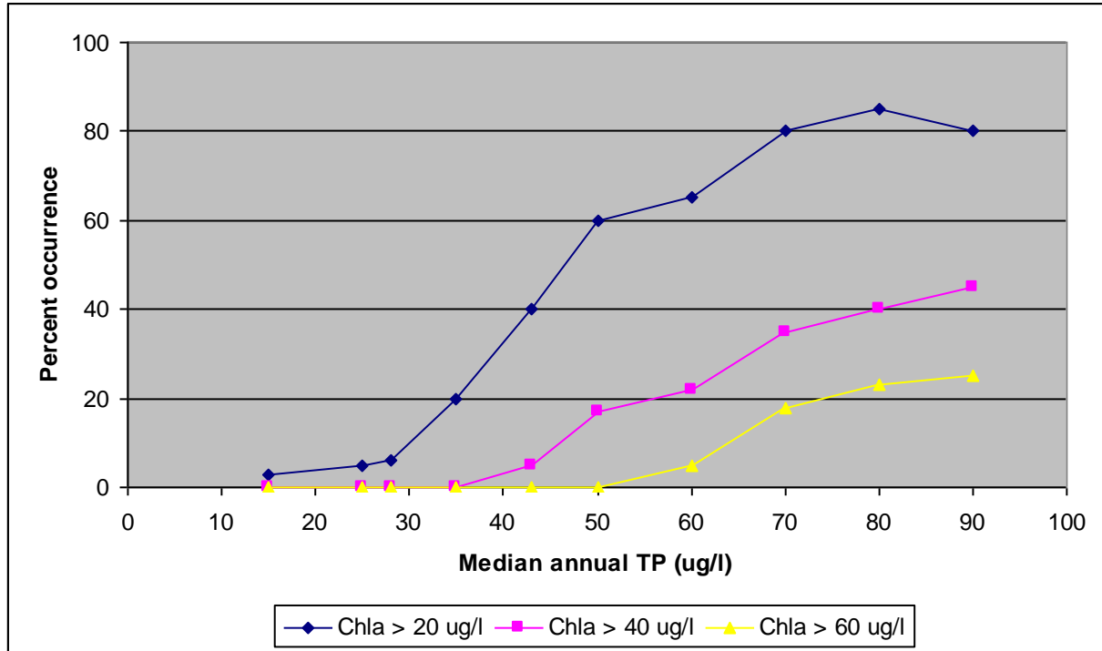
Figure 2-1(L2) Percent occurrence of chlorophyll-a concentrations in excess of specified levels as a function of total phosphorous (example)
