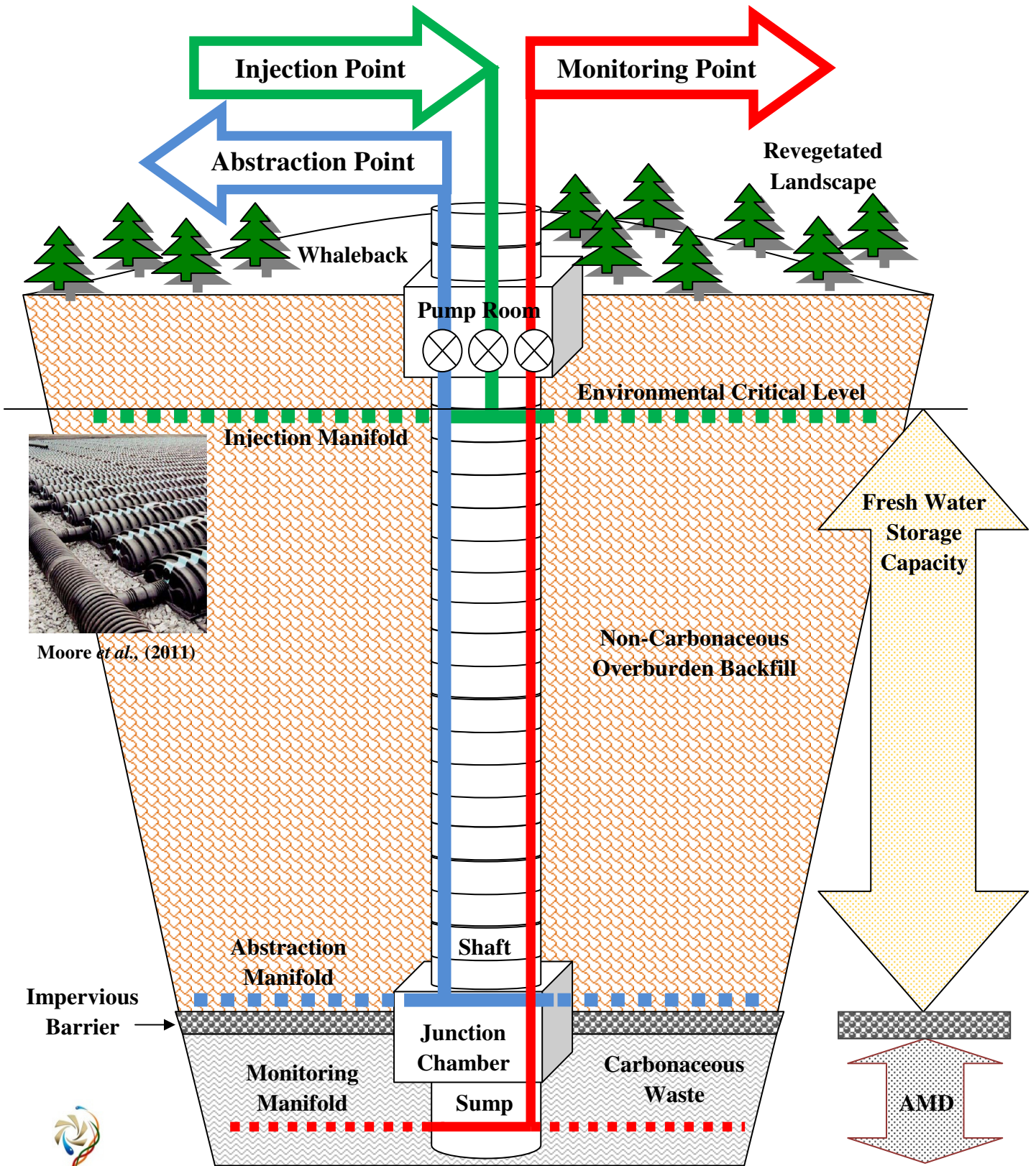
AMD Dual Stream Reticulation Schematic Rehabilitated Open Cast Coal Pit
